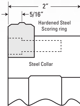
Drawing shows how scoring ring is adapted to collar for quick, accurate set-up
